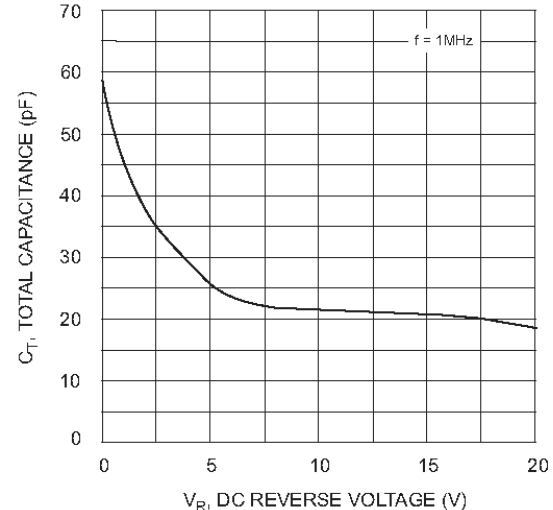
V_R , DC REVERSE VOLTAGE (V) Fig. 4 Typ. Total Capacitance vs Reverse Voltage
